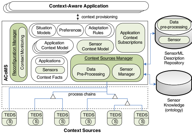
Fig. 4. Open Context-Aware System Architecture
